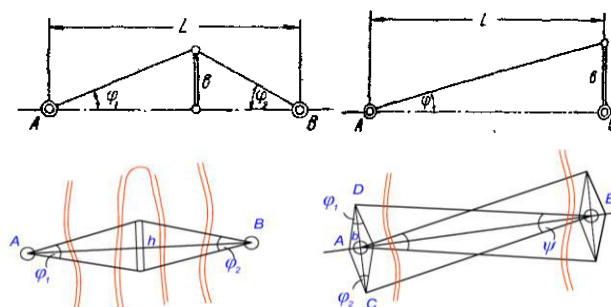
Figure 2. Parallax units used in measuring bridge spans
