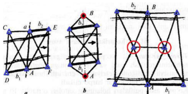
Figure 4. Bridge triangulation
